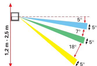
Ranges and detection angles
