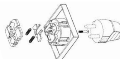
Explosion diagram: SCHUKO® child protection socket outlet
