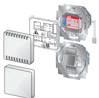
Explosion diagram room thermostat object range
